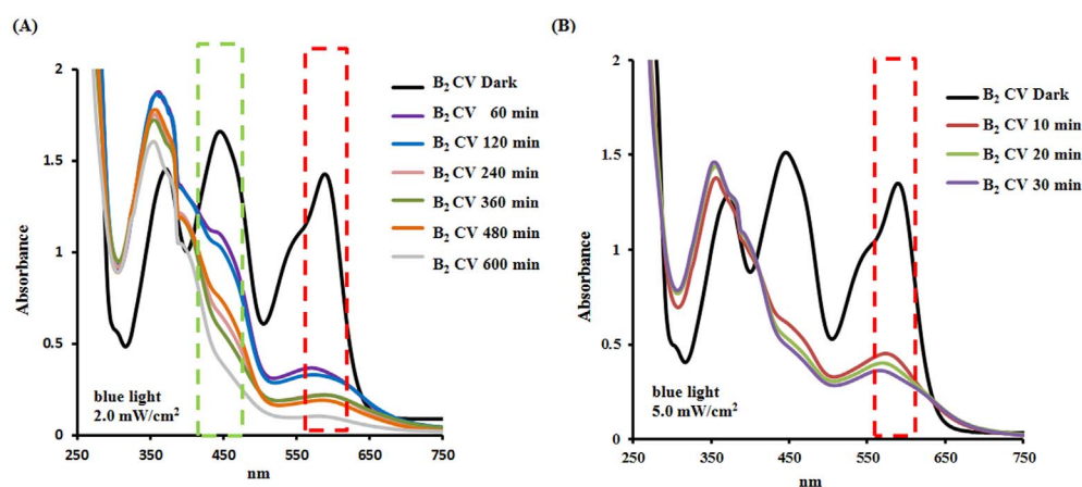
Fig. 6. (A) The absorbance spectra of CV in 240 \mu\text{M} riboflavin ( \text{B}_2 ) solution treated with blue light irradiation at 2.0 \text{mW}/\text{cm}^2 for 60, 120, 240, 360, 480 and 600 min. (B) The absorbance spectra of CV in 240 \mu\text{M} riboflavin solution treated with blue light irradiation at 5.0 \text{mW}/\text{cm}^2 for 10, 20 and 30 min. (For interpretation of the references to color in this figure legend, the reader is referred to the web version of this article.)
