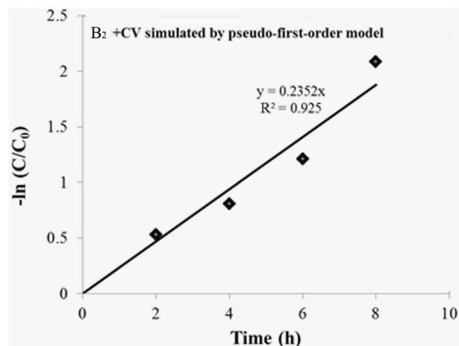
Fig. 7. Pseudo first-order apparent degradation rate constants of CV at initial riboflavin ( \text{B}_2 ) concentration of 240 \mu\text{M} , treated with blue light irradiation at 2.0 \text{W}/\text{cm}^2 .
