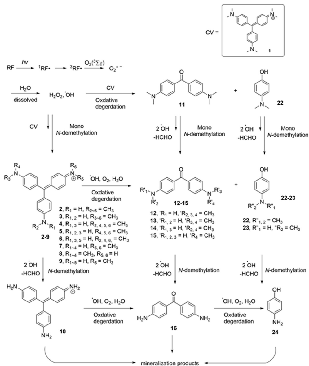
Fig. 9. Scheme for the photodegradation mechanisms of RF/CV.
