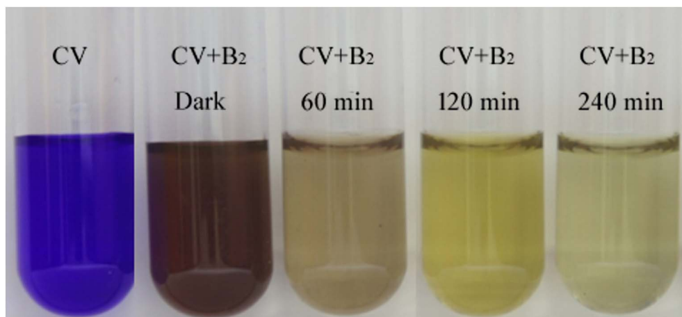
Fig. 5. Color changes of CV in 240 \mu\text{M} riboflavin ( \text{B}_2 ) solution treated with blue light irradiation at 2.0 \text{mW}/\text{cm}^2 for 60, 120, and 240 min. (For interpretation of the references to color in this figure legend, the reader is referred to the web version of this article.)
