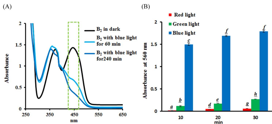
Fig. 2. (A) 240 \mu\text{M} riboflavin illuminated by blue light irradiation at 2.0 \text{ mW}/\text{cm}^2 for 60 and 240 min. (B) Effects of light quality on NBT reduction by riboflavin ( \text{B}_2 ) photolysis at 2.0 \text{ mW}/\text{cm}^2 with irradiation for 10, 20, and 30 min. Data were represented by mean \pm SD, where n = 3 . Significant differences ( p < 0.05 ) between groups are indicated by the different letters above each bar.
