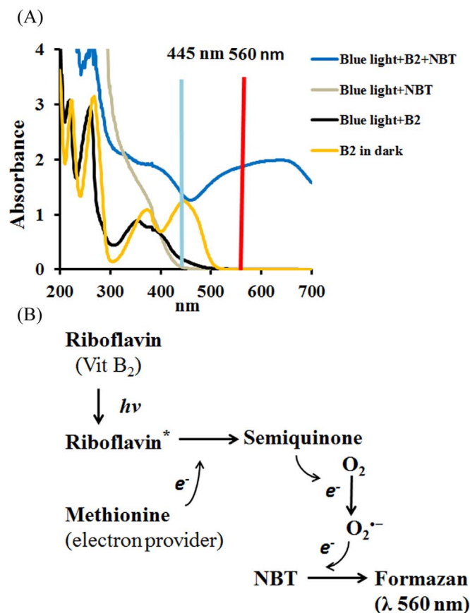
Fig. 3. (A) Spectra of B 2 /NBT method upon irradiation by a blue LED at 2.0 \text{ mW}/\text{cm}^2 for 30 min. (B) The generated \text{O}_2^{\cdot-} from riboflavin ( \text{B}_2 ) photolysis and assayed by measuring the photoreduction of nitro blue tetrazolium (NBT). (For interpretation of the references to color in this figure legend, the reader is referred to the web version of this article.)
