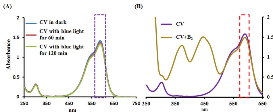
Fig. 1. Spectra of (A) 10 µg/g CV illuminated by blue light irradiation at 2.0 mW/cm 2 for 60 and 120 min, respectively, and (B) 10 µg/g CV alone and CV in 240 µM riboflavin (B 2 ) solution. (For interpretation of the references to color in this figure legend, the reader is referred to the web version of this article.)
