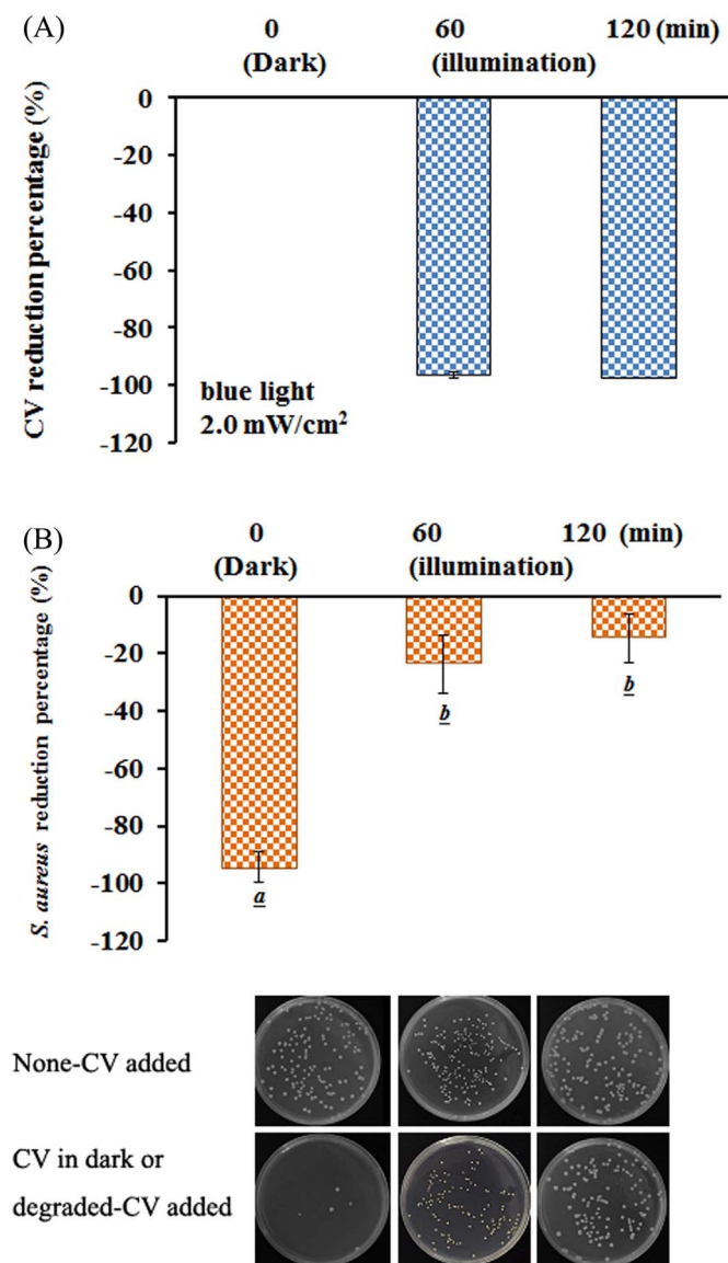
Fig. 8. (A) Effects of riboflavin photolysis on CV degradation. The reduction percentage was the degradation of CV in a riboflavin solution after treatment with blue light irradiation at 2.0 mW/cm 2 for 60 and 120 min, as detected by an HPLC system at 588 nm. (B) Effects of CV or degraded CV in riboflavin solution on viability of S. aureus . CV of 10 mg/L in the dark without blue light irradiation was used as a control. Other treatments were 10 mg/L CV in riboflavin solution treated with blue light irradiation at 2.0 mW/cm 2 for 60 and 120 min. Data are represented by mean \pm SD, where n = 5 . Statistical differences ( p < 0.05 ) between groups are indicated by the different letters below each bar. (For interpretation of the references to color in this figure legend, the reader is referred to the web version of this article.)
