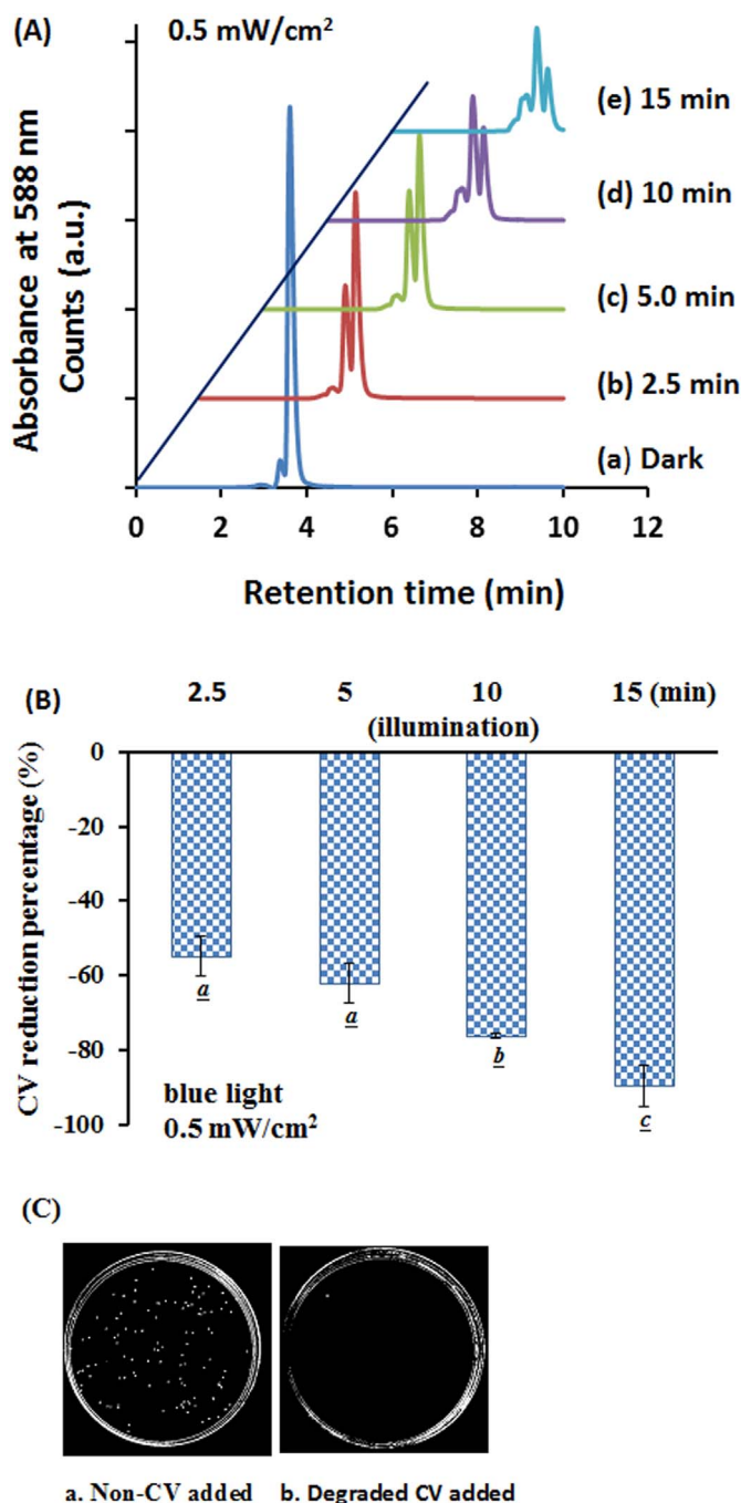
Fig. 4. (A) Chromatograms of 25 mg/L CV in riboflavin ( B_2 ) solution treated with blue light irradiation. The chromatogram of CV without blue light irradiation is shown in line (a) as a control. Other chromatograms represent those treated with blue light irradiation for (b) 2.5, (c) 5.0, (d) 10, and (e) 15 min. (B) Effects of riboflavin photolysis on CV degradation. The reduction percentage was the degradation of CV in a riboflavin solution after treatment with blue light irradiation at 0.5 mW/cm 2 for 2.5, 5, 10, and 15 min, as detected by an HPLC system at 588 nm. (C) Effects of degraded CV in riboflavin solution on viability of S. aureus . 25 mg/L of CV in riboflavin solution was treated with blue light irradiation at 0.5 mW/cm 2 for 15 min. Data were represented by mean \pm SD, where n = 3 . Statistical differences ( p < 0.05 ) between groups are indicated by the different letters below each bar. (For interpretation of the references to color in this figure legend, the reader is referred to the web version of this article.)
